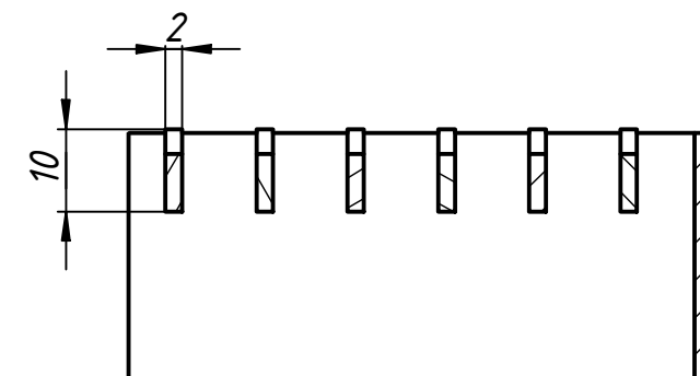
B-B (1:1)
